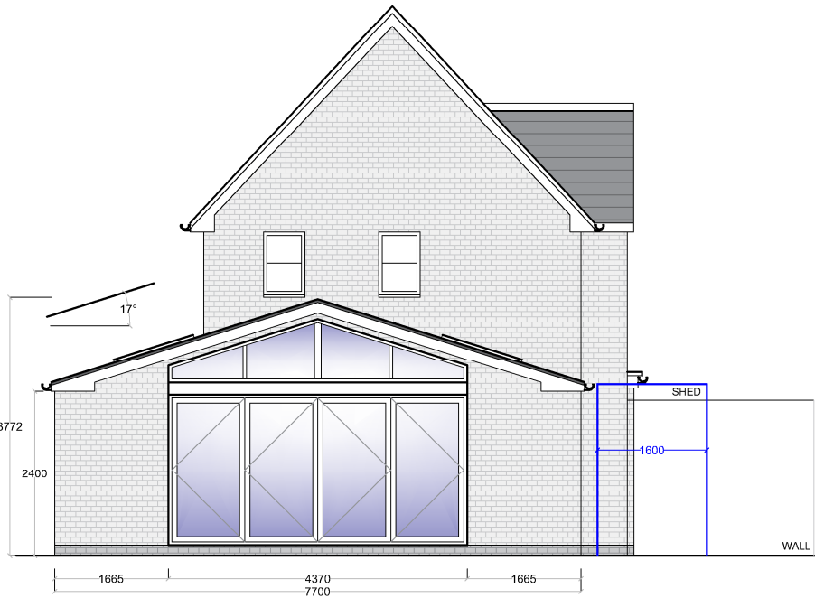
PROPOSED SIDE ELEVATION (Scale 1:100) SCALE BAR - (mm) 500 1000 2000
