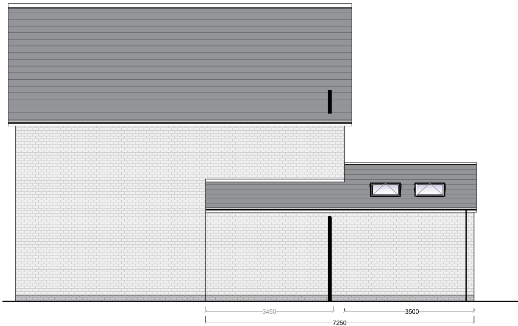
PROPOSED REAR ELEVATION (Scale 1:100) SCALE BAR - (mm) 500 1000 2000
