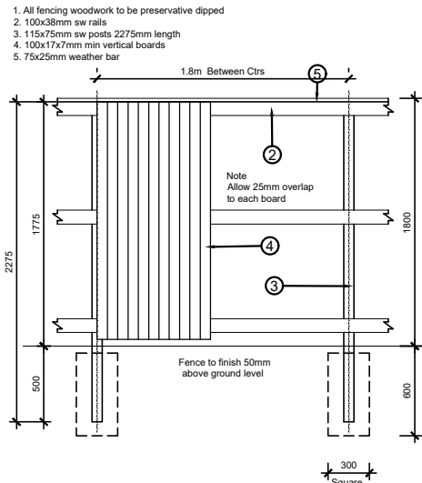
1800mm High Heavy Duty Vertical Lap Fence or Featheredge (3)
