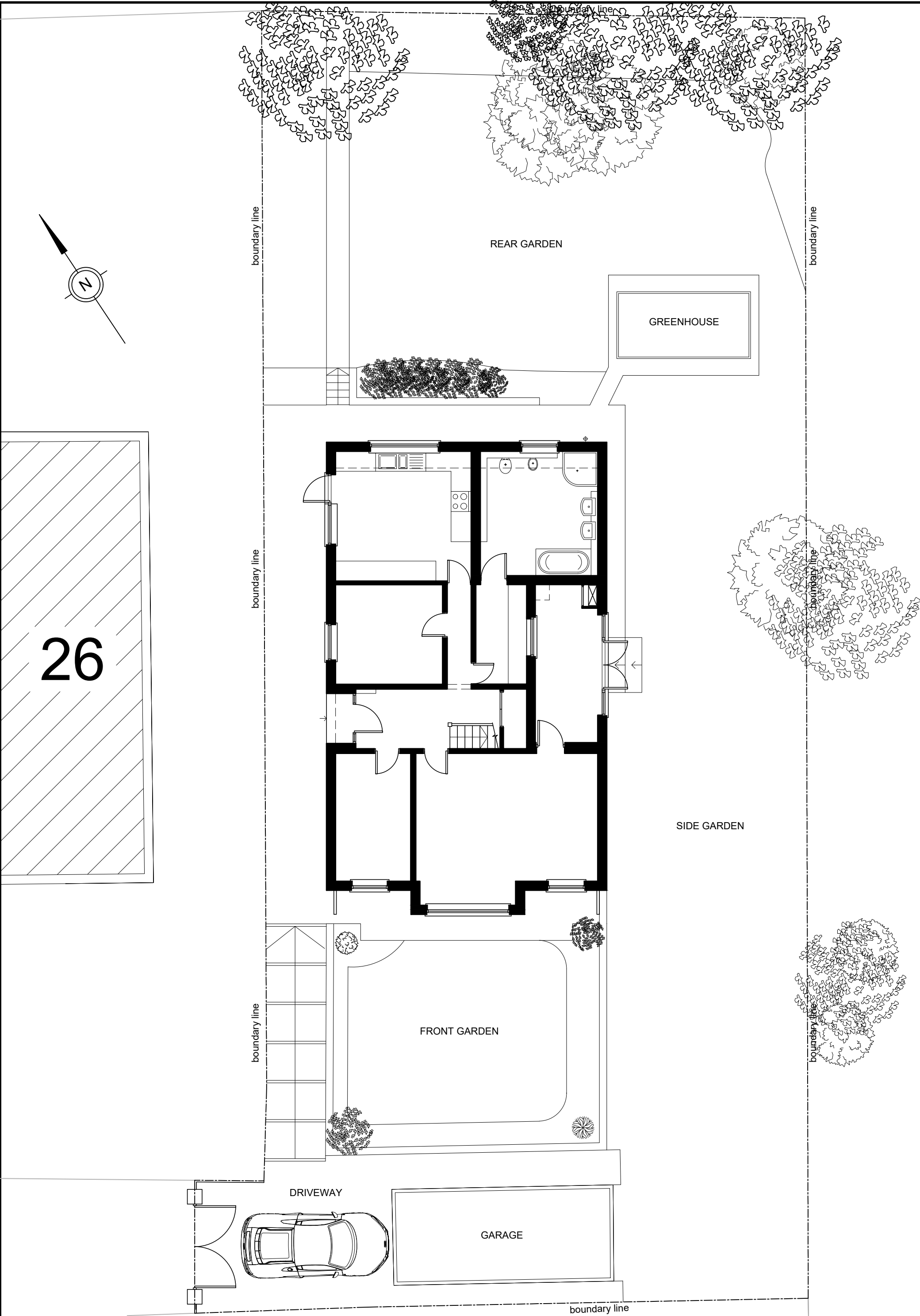
1:100 scale bar 0 1 2 3 4 5metres EXISTING SITE BLOCK PLAN
