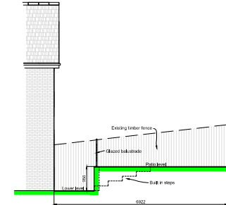
Current Patio Cross Section
