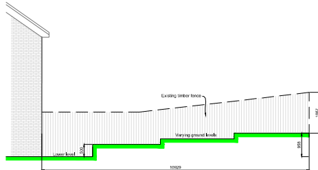
Former Garden Cross Section
