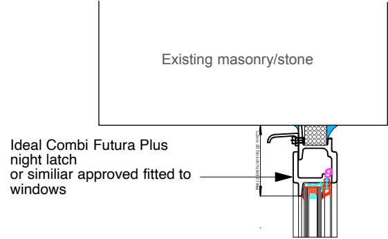
Detail 10 (scale 1:5)
