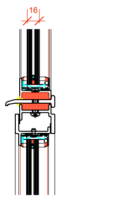
Detail 14 (scale 1:5)
