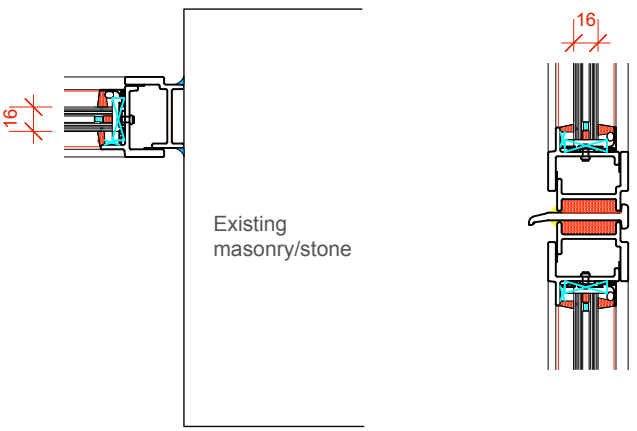
Detail 19 (scale 1:5)
