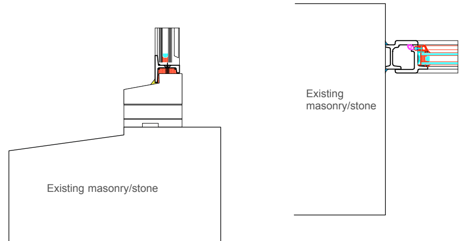
Detail 02 (scale 1:5)
