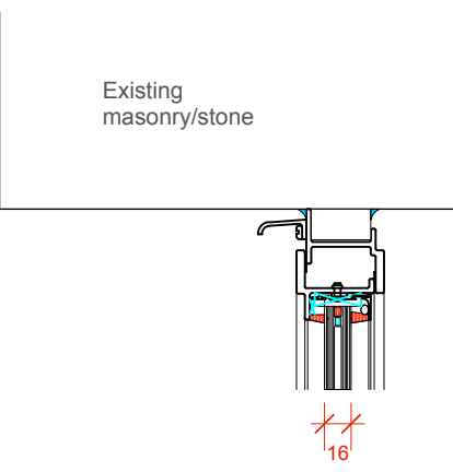
Detail 20 (scale 1:5)
