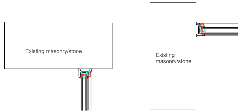
Detail 01 (scale 1:5)
