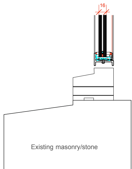
Detail 12 (scale 1:5)
