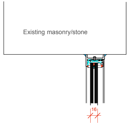
Detail 11 (scale 1:5)
