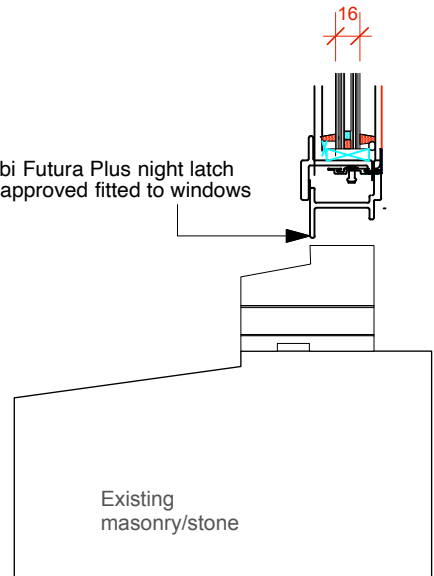
Detail 18 (scale 1:5)
