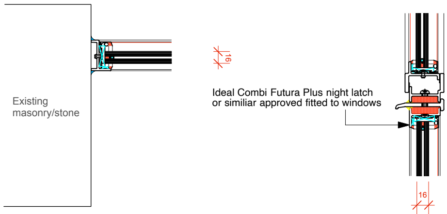
Detail 13 (scale 1:5)
