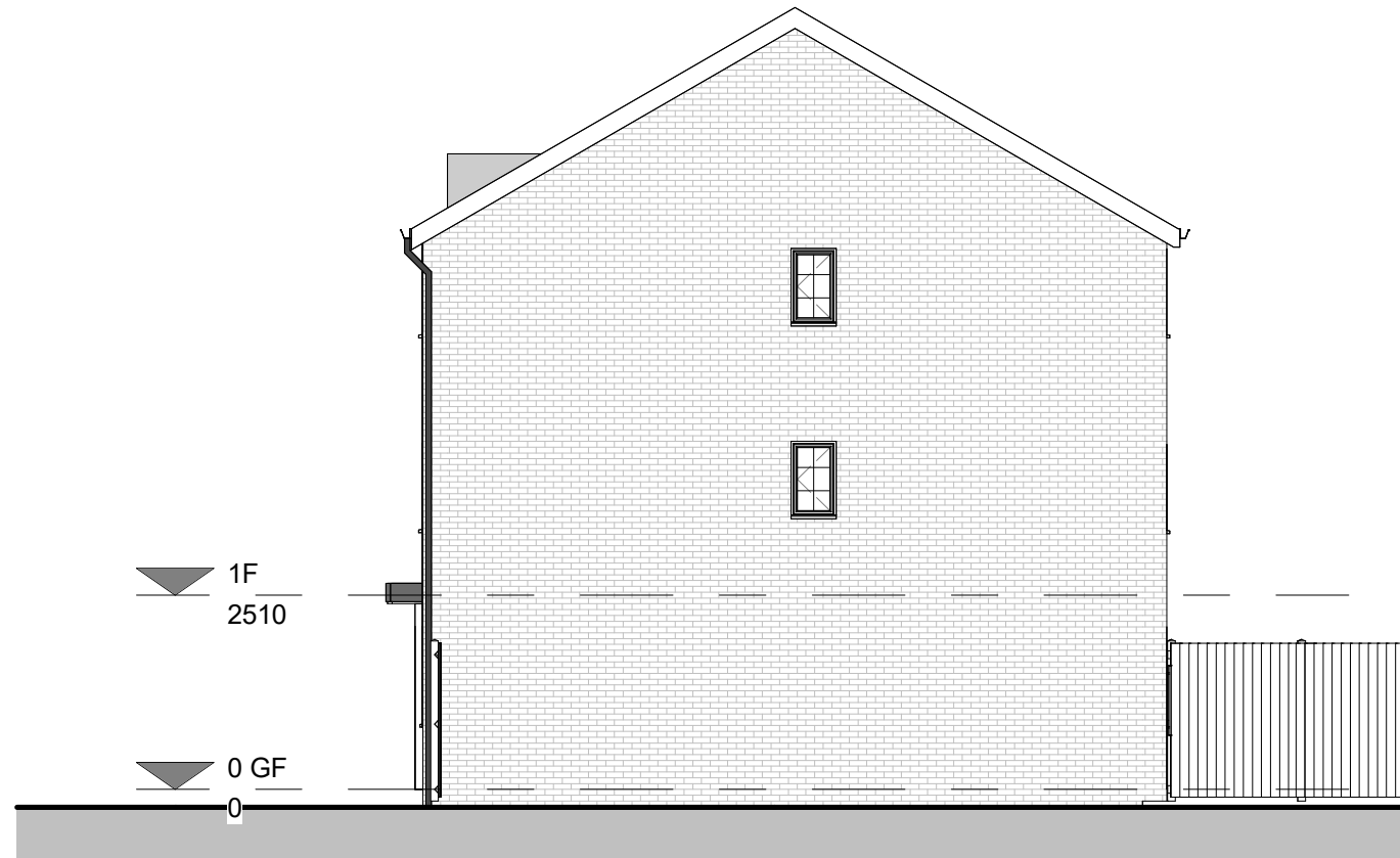
SIDE ELEVATION I (East Facing)
