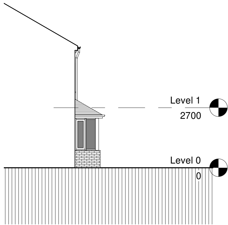
West Elevation 1 : 100
