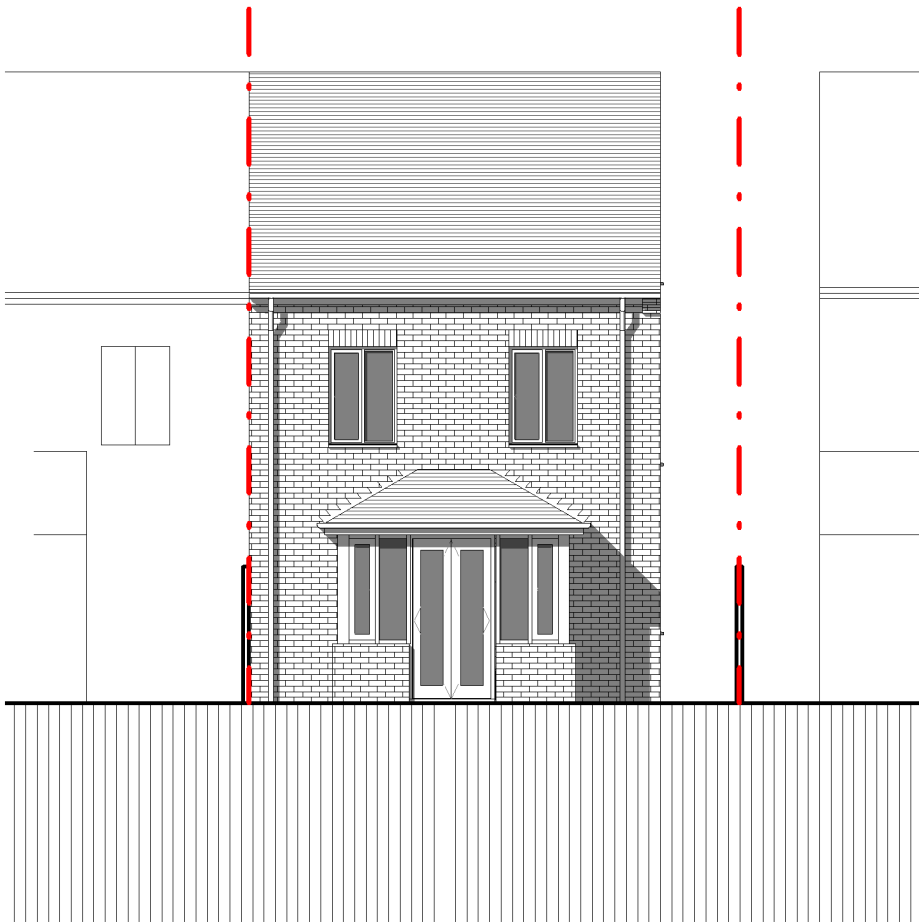
South Elevation 1 : 100
