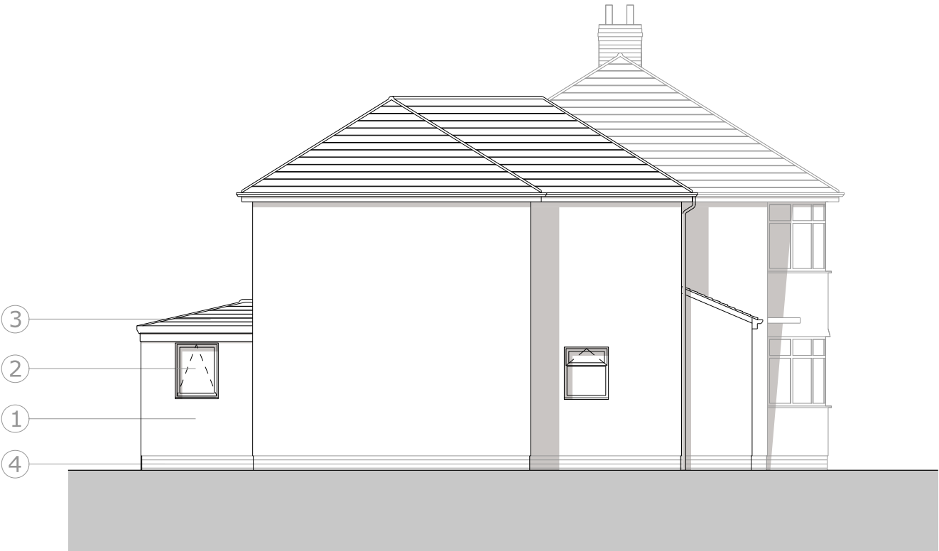
Proposed Gable End Elevation
