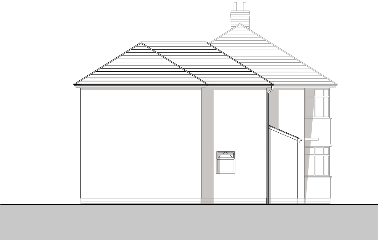
Existing Gable End Elevation
