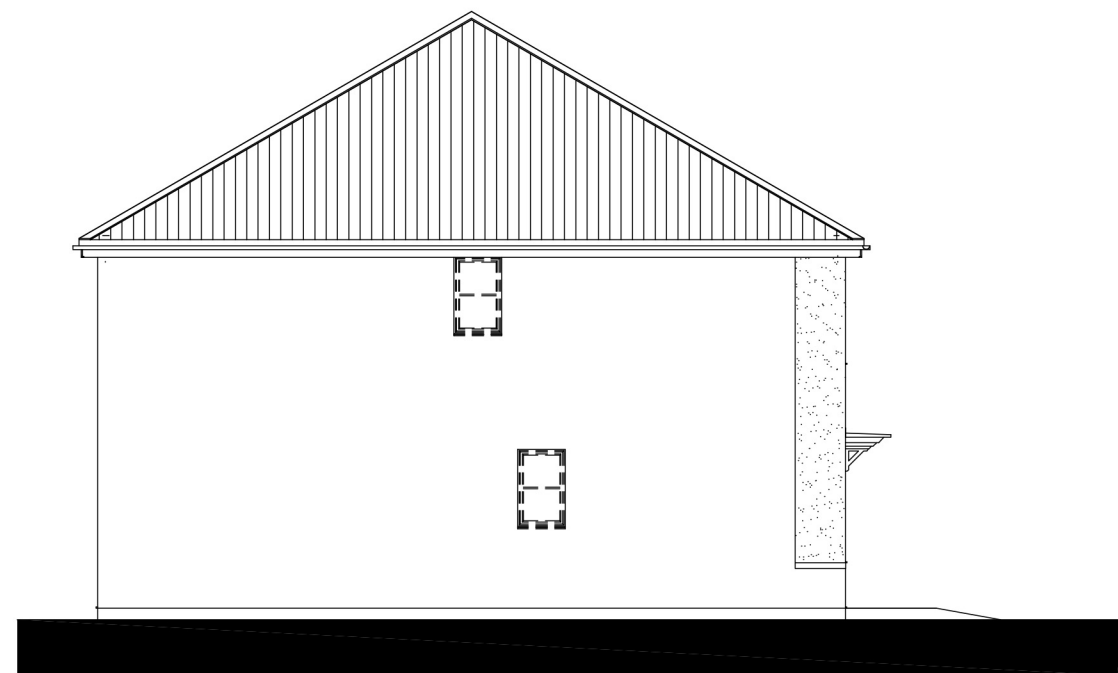
REAR ELEVATION
