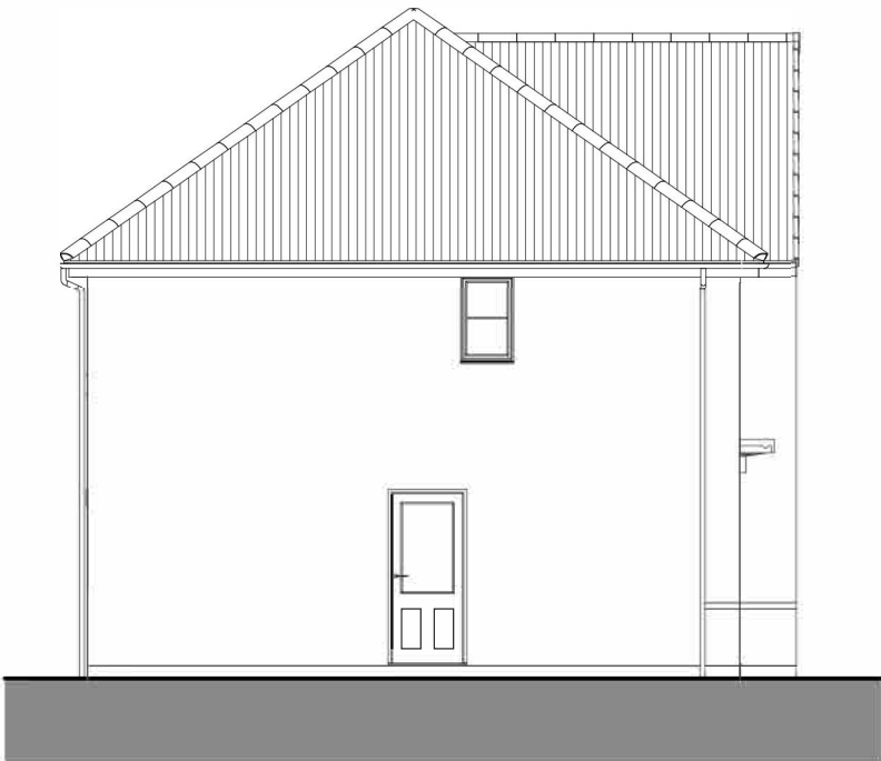
SIDE ELEVATION
