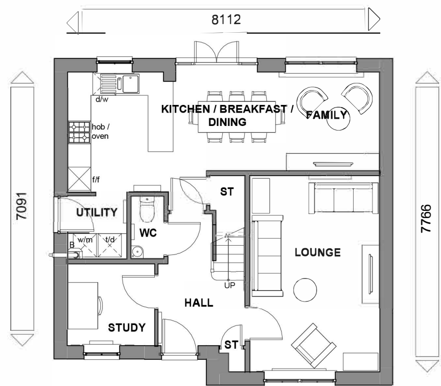
GROUND FLOOR
