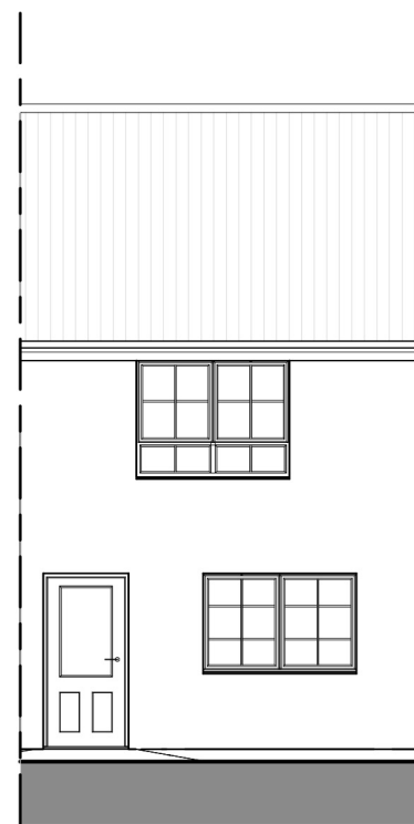
REAR ELEVATION
