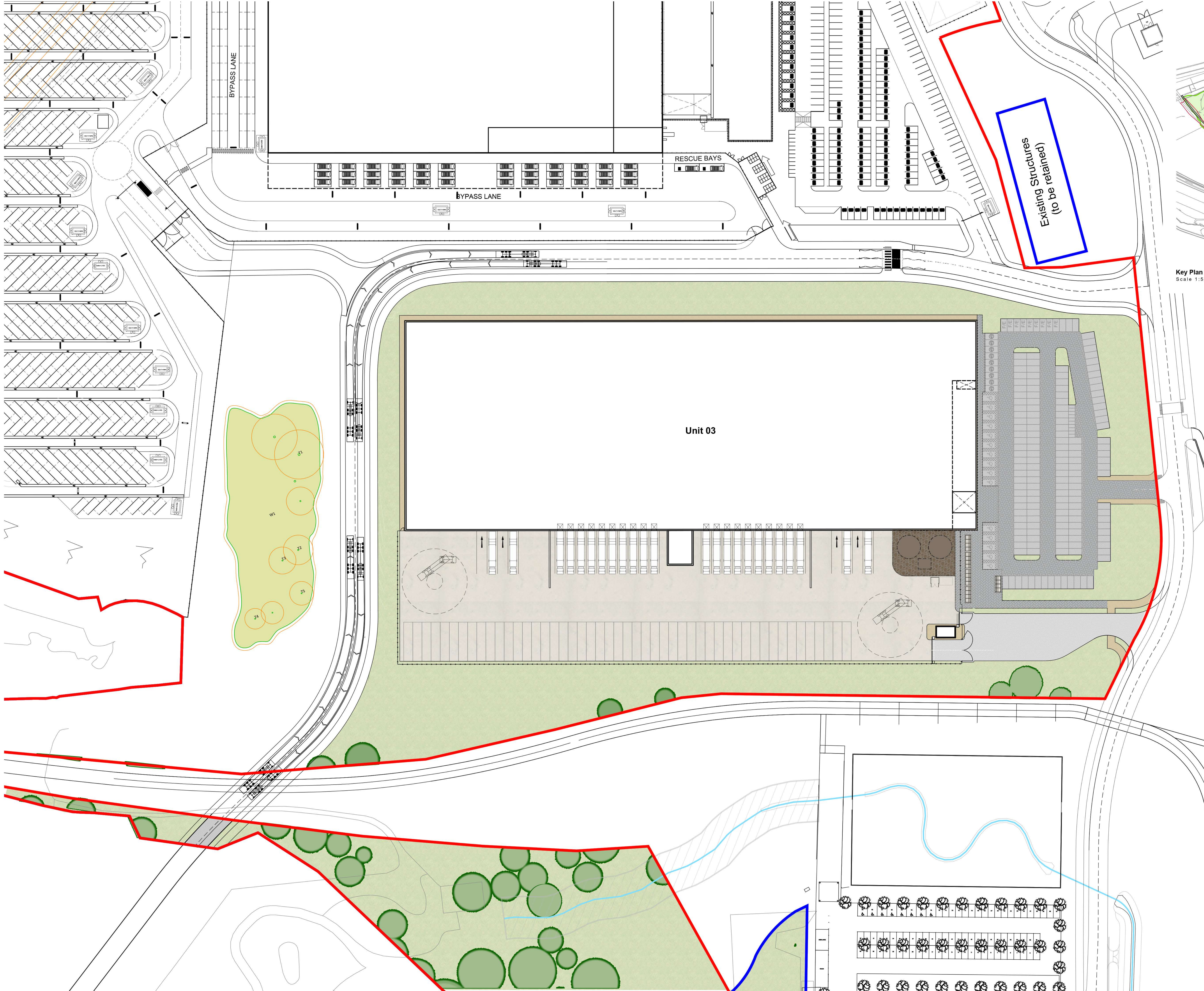
Unit 3 - External Finishes Plan Scale 1:500
