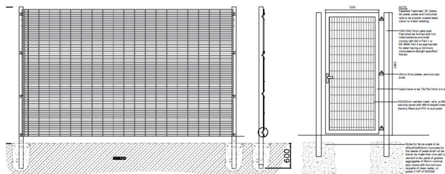
(Typical fence and gate elevation)
