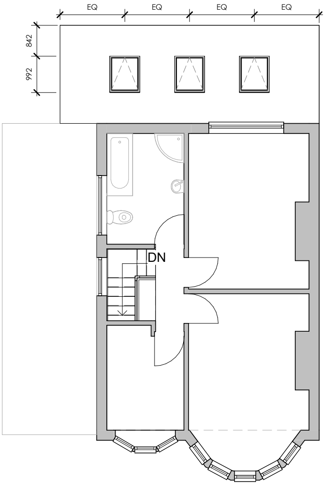
FIRST FLOOR PLAN - PROPOSED @1:100
