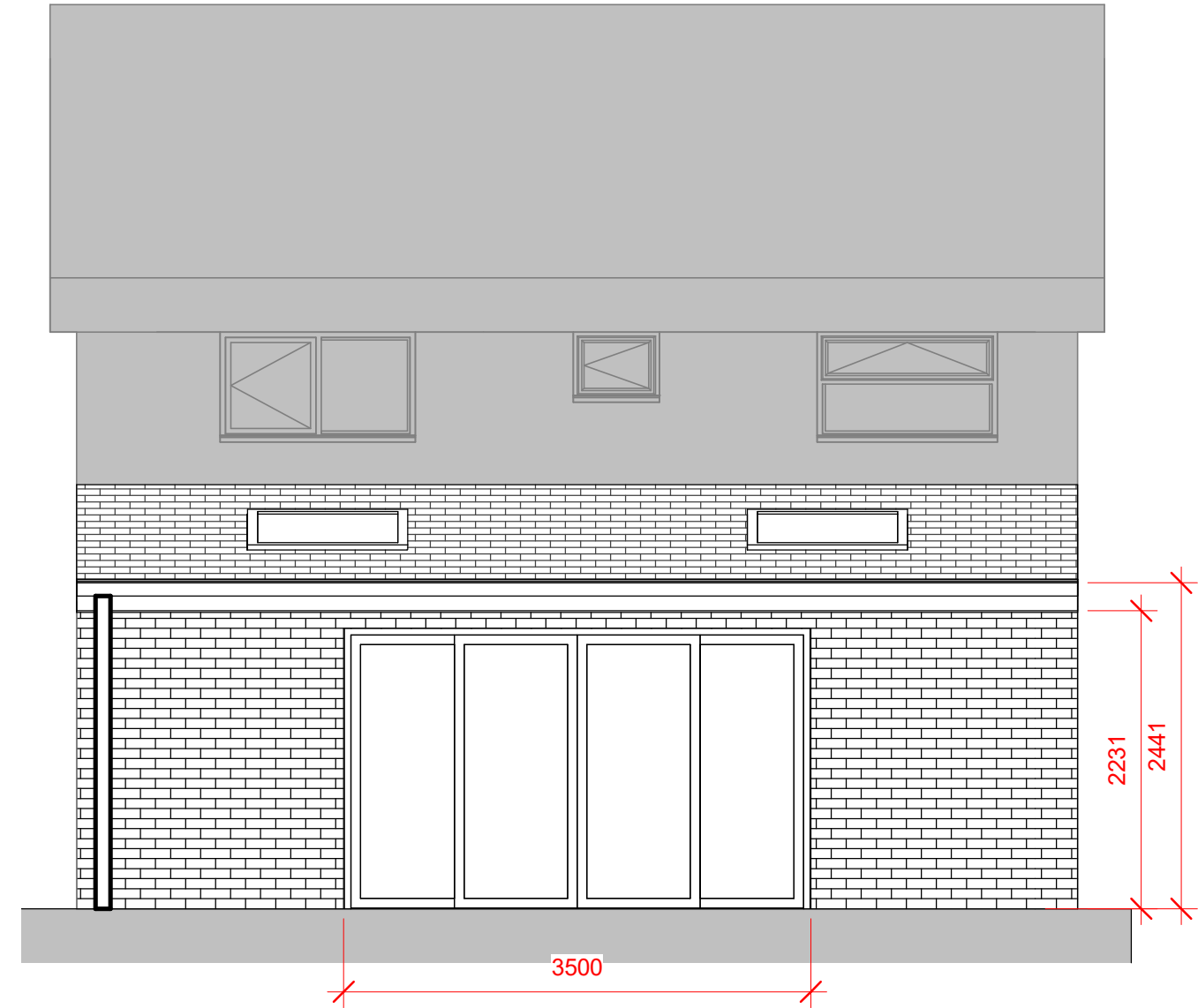
Rear Elevation 1 : 50
