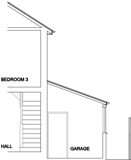
SECTION B-B (EXISTING)
