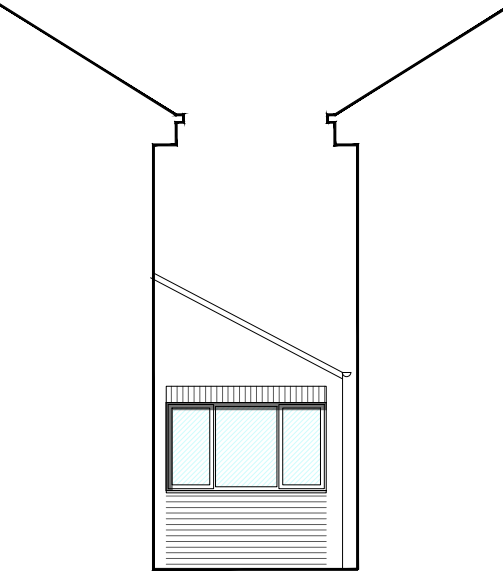
Proposed Part Front Elevation Scale 1:100 (Play Room)
