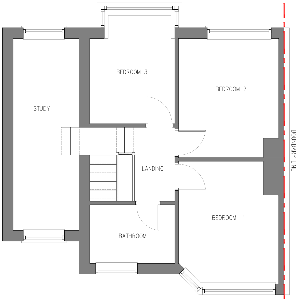
EXISTING FIRST FLOOR | SCALE 1:50
