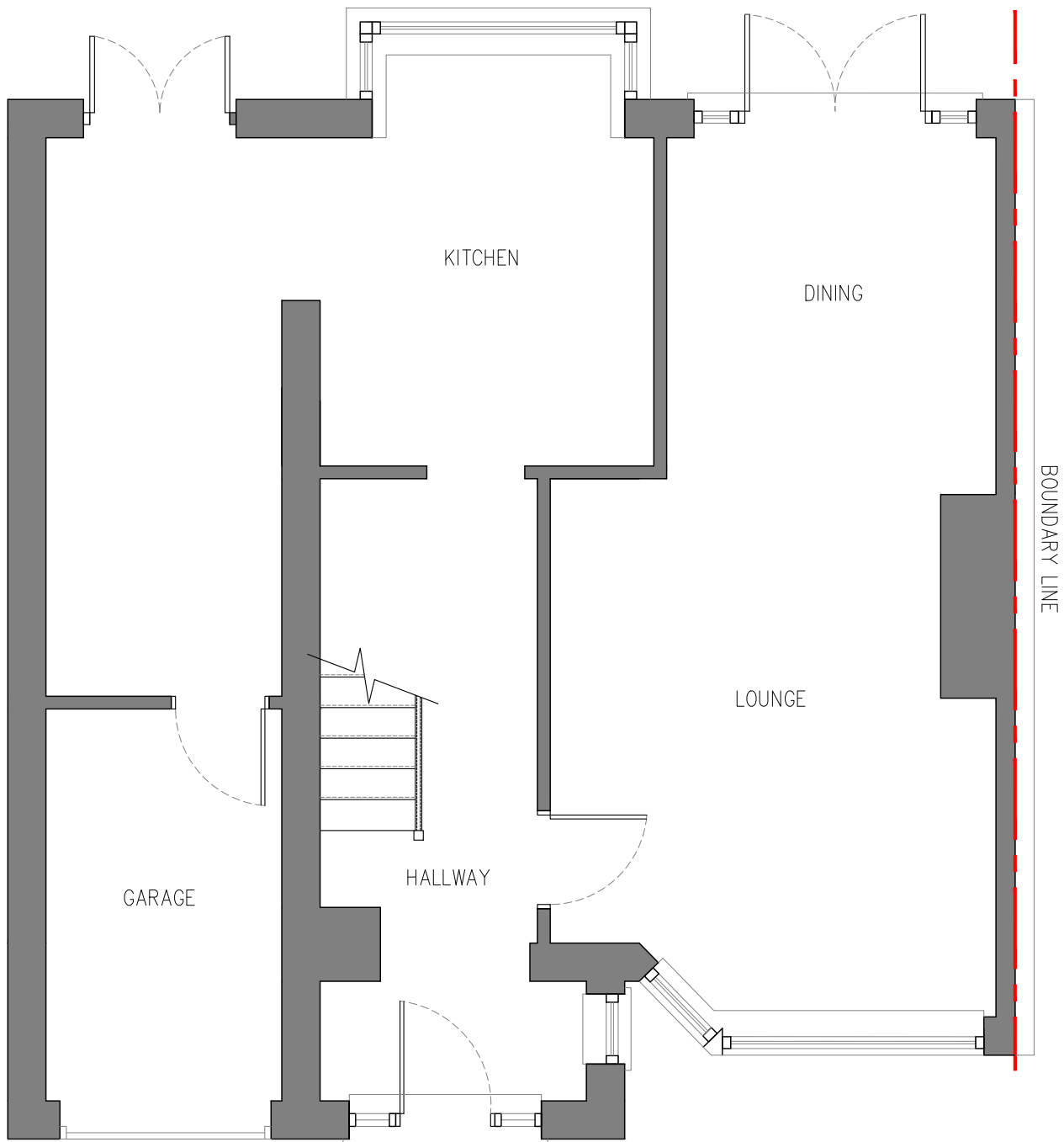
EXISTING GROUND FLOOR | SCALE 1:50
