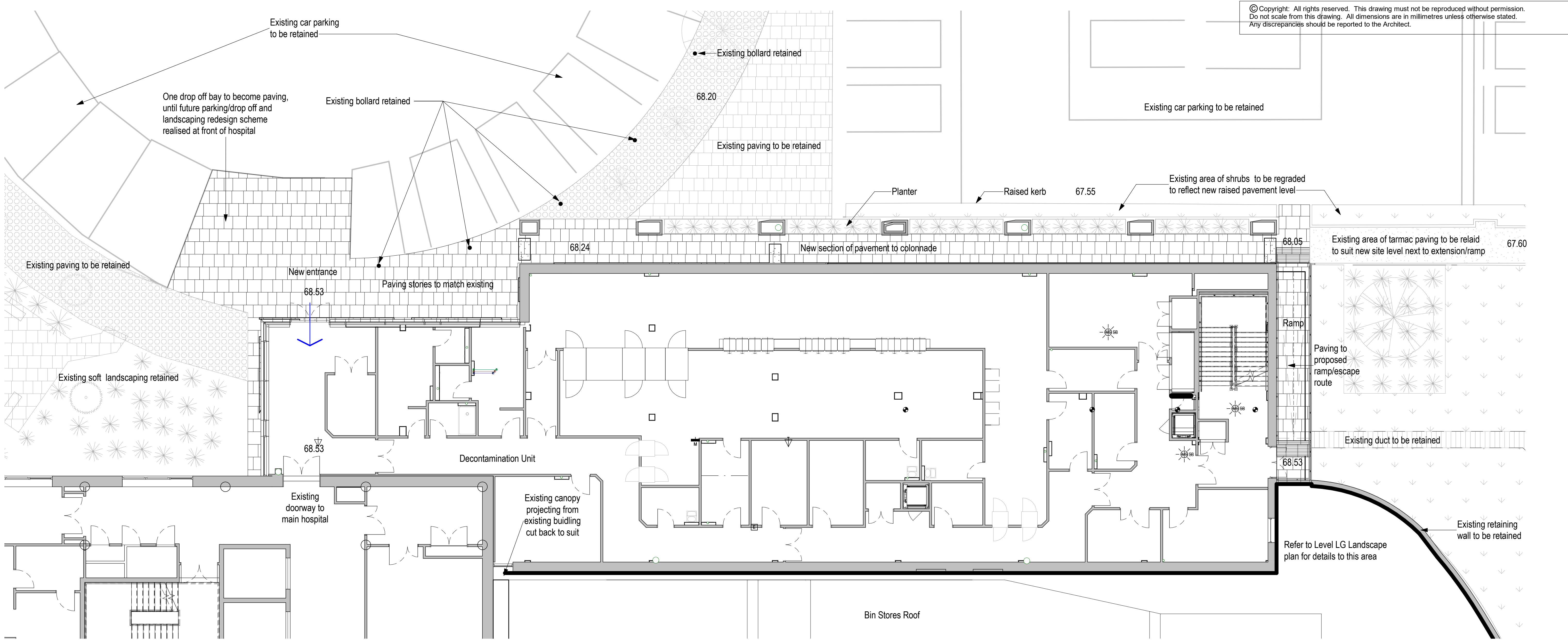
Level 1 Proposed Landscape Plan
