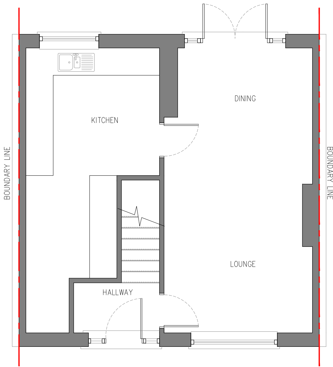
EXISTING GROUND FLOOR | SCALE 1:50
