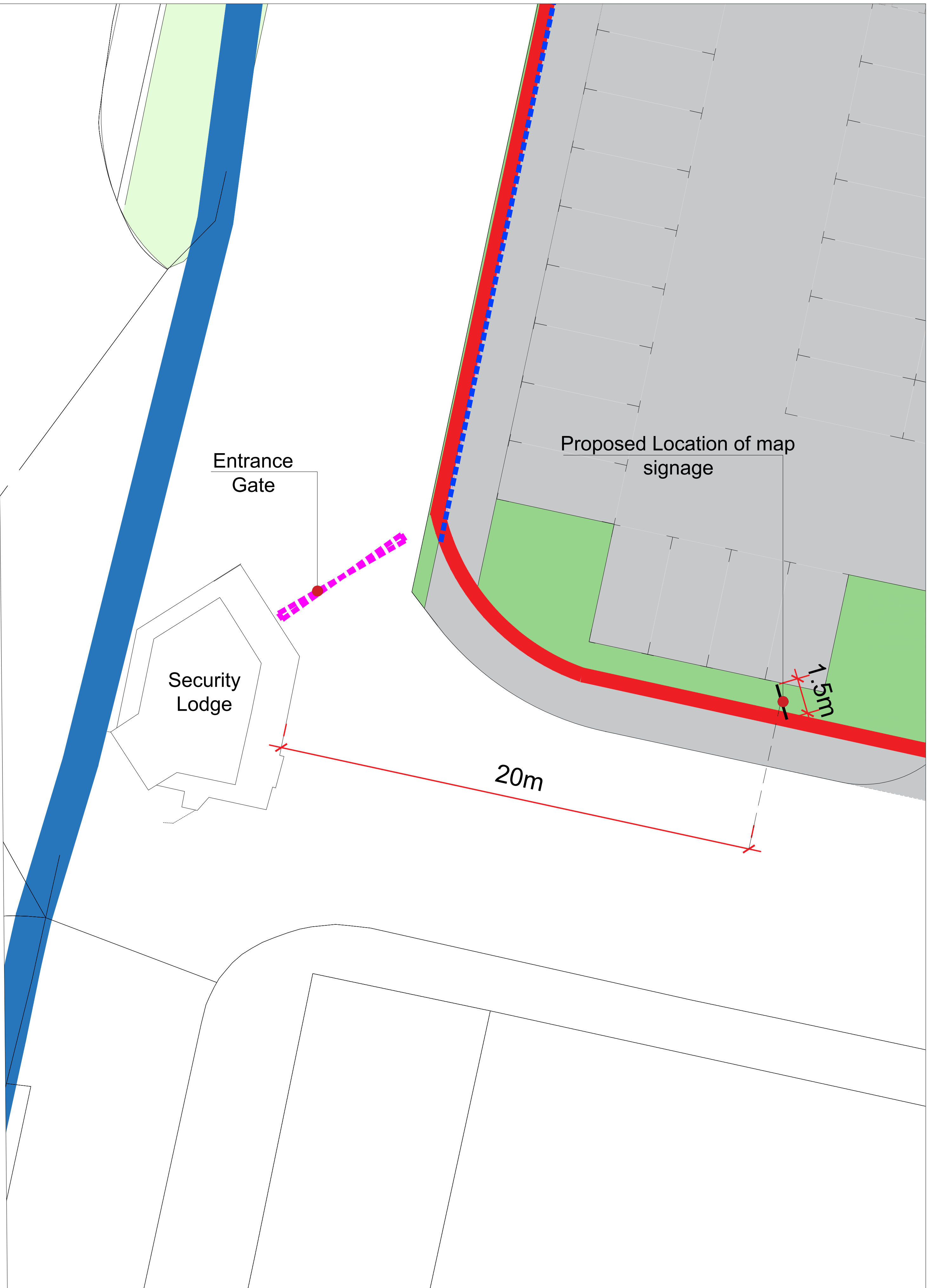
02 Site Entrance Signage Plan 1:100 @ A1
