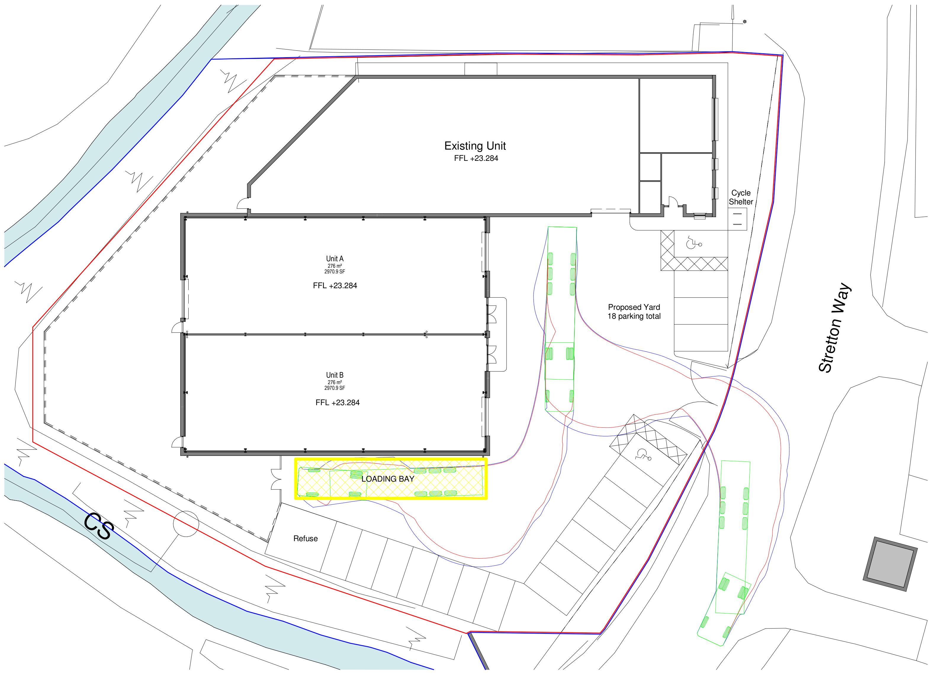
HGV Tracked Egress 1 : 200
