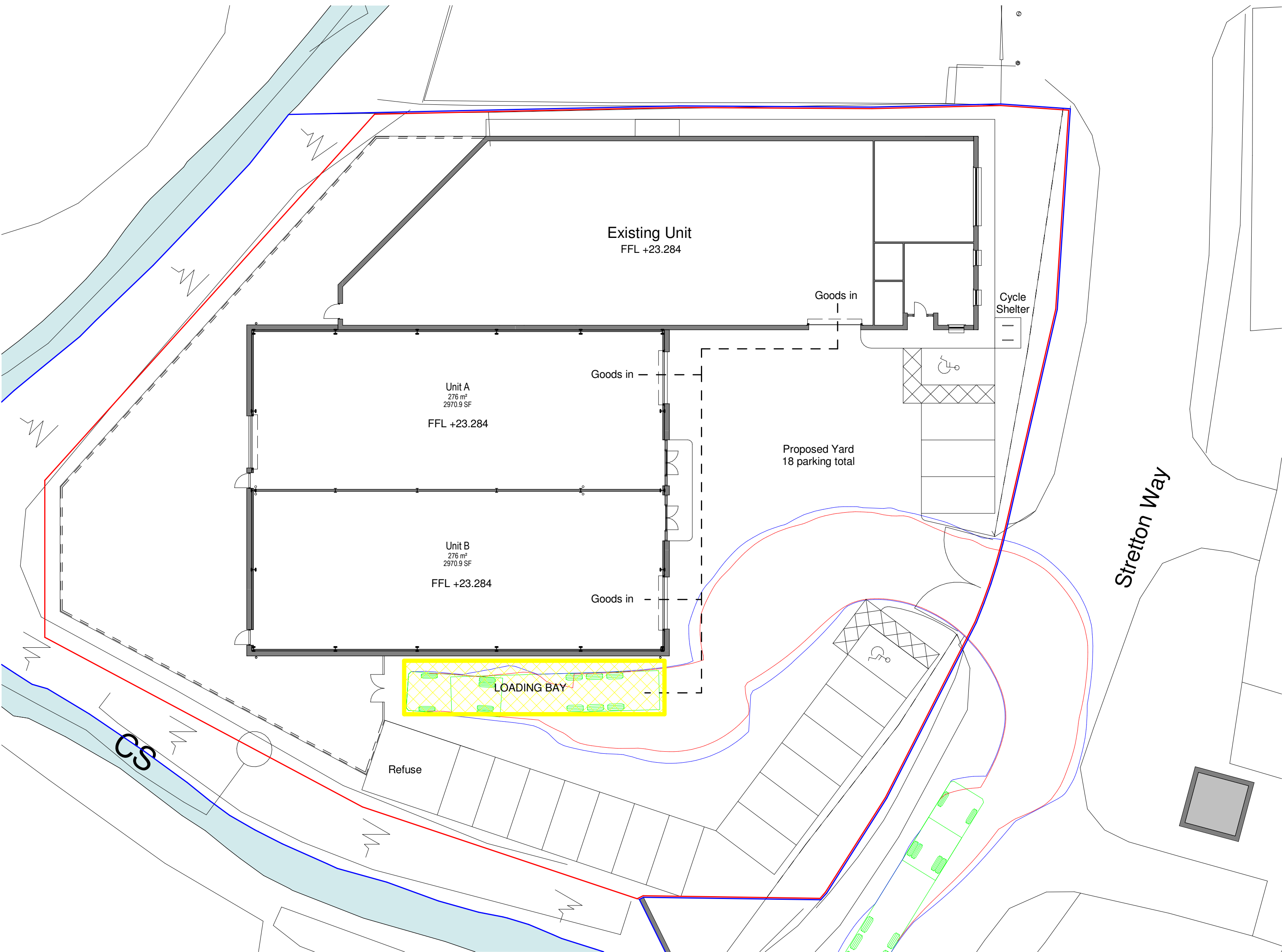
HGV Tracked Ingress 1 : 200
