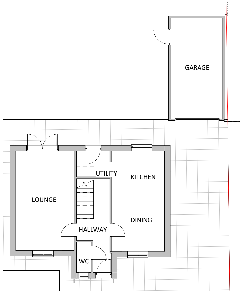
GROUND FLOOR PLAN 1:100@A3
