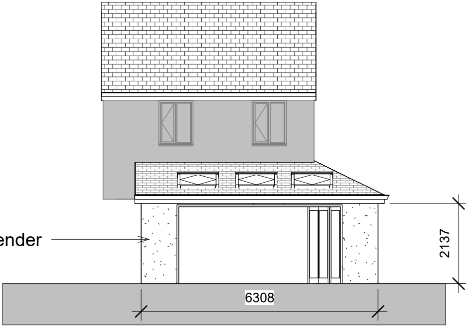
Rear Elevation 1 : 100
