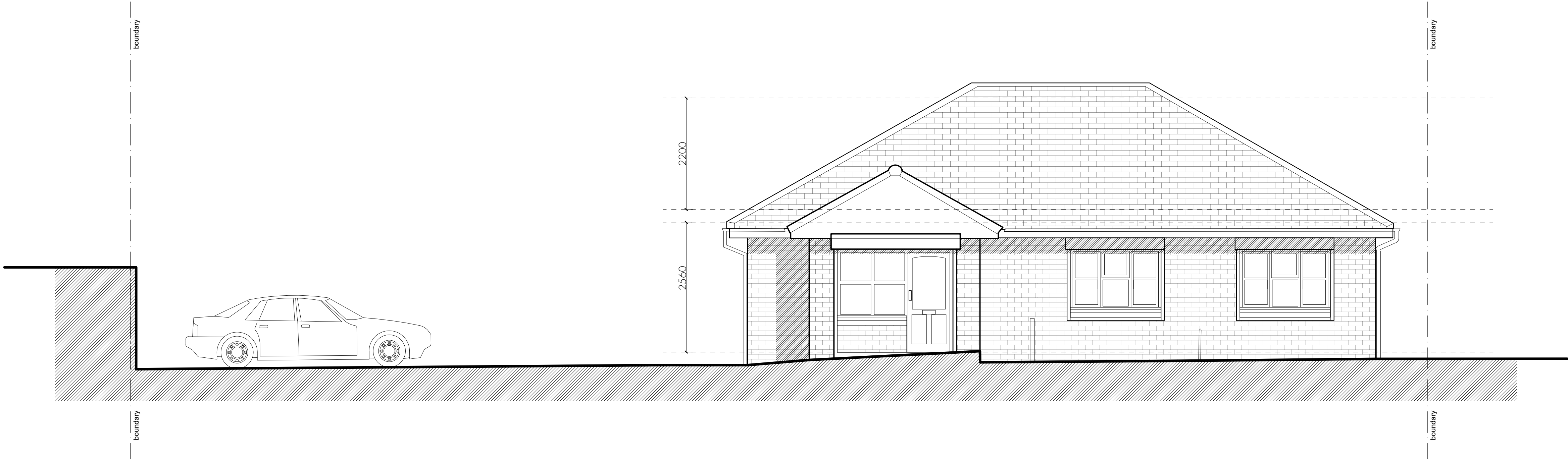
PROPOSED FRONT ELEVATION 1:50 Scale
