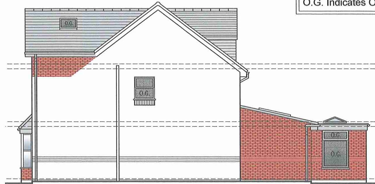
Proposed Side Elevation. West Facing
