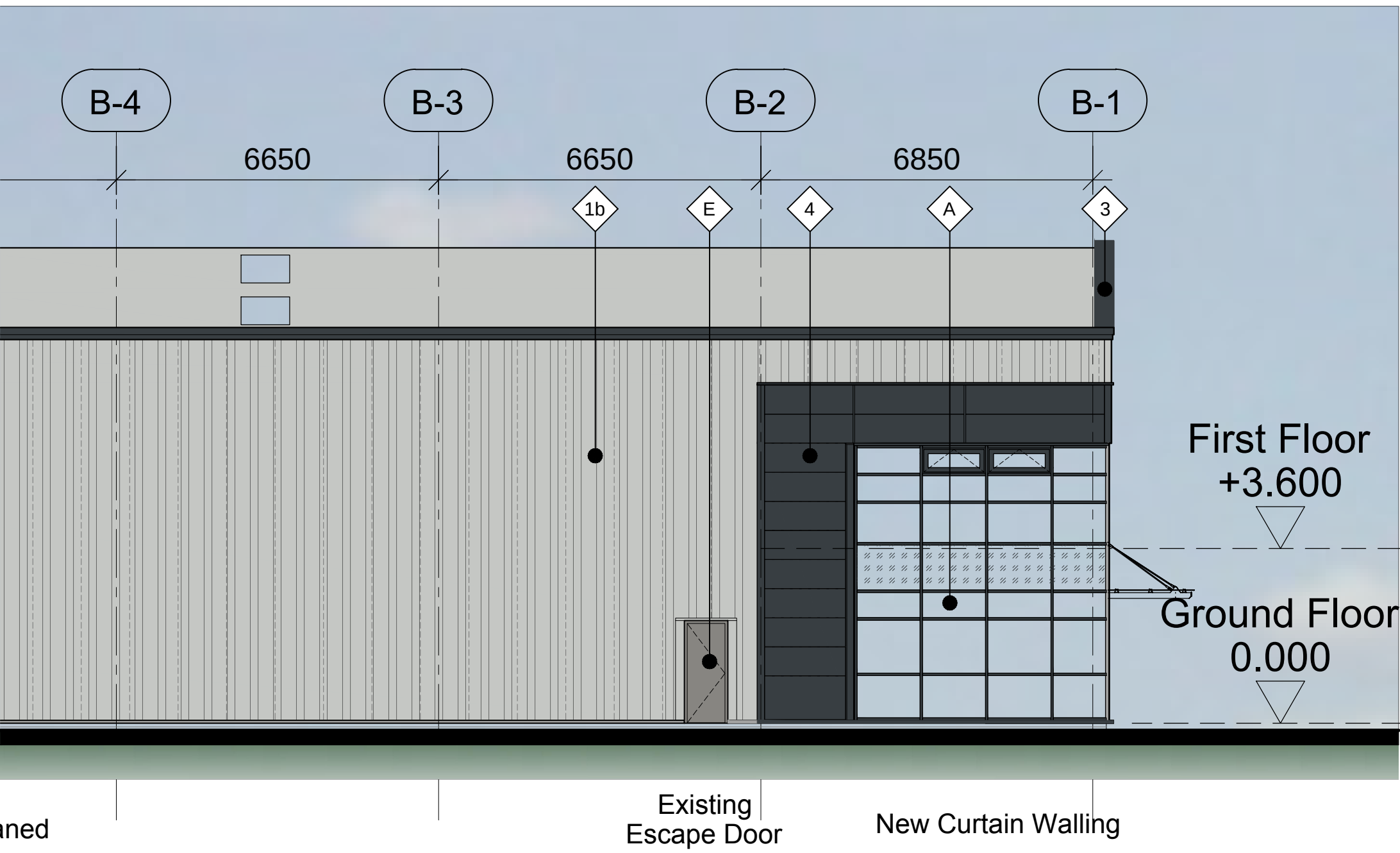
South Elevation - continued below
