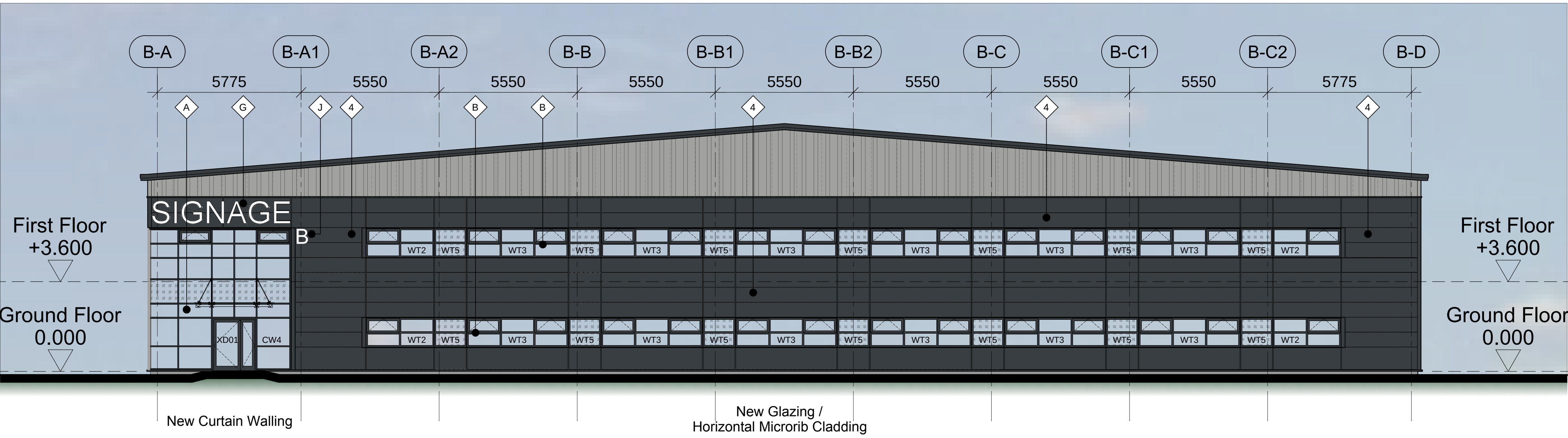
East Elevation (towards Entrance)
