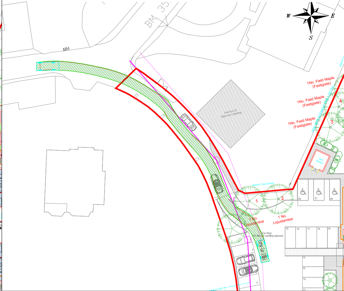
LARGE CAR TRACKS WITHIN CAR PARK
