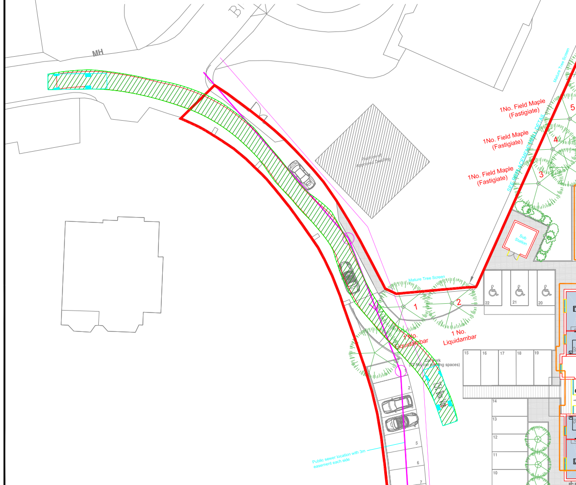
RIGID DELIVERY VEHICLE EGRESS WITH LARGE CAR IN PASS-BY
