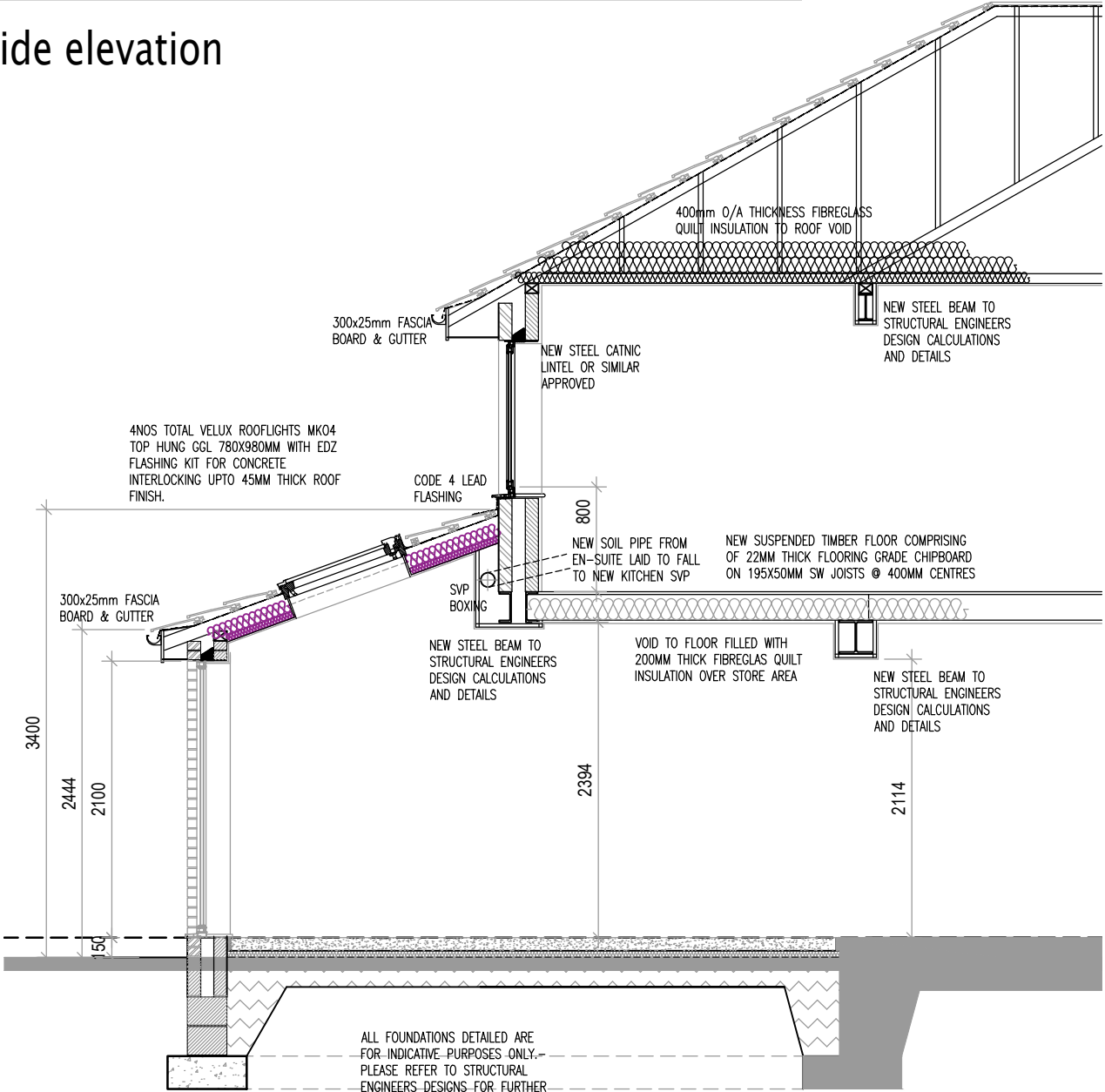
Proposed cross section (partial)
