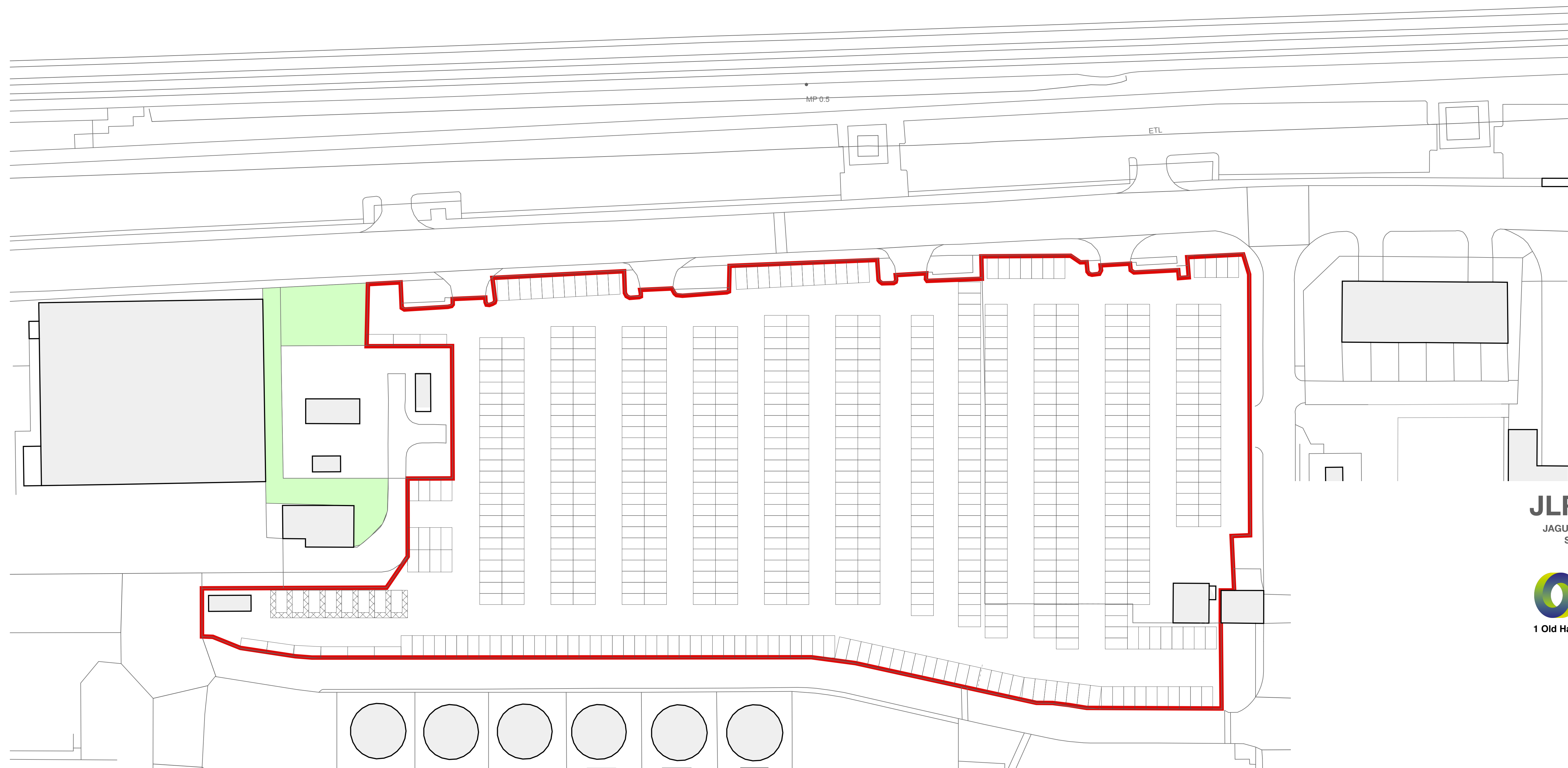
SITE E - BLOCK PLAN 1:500
