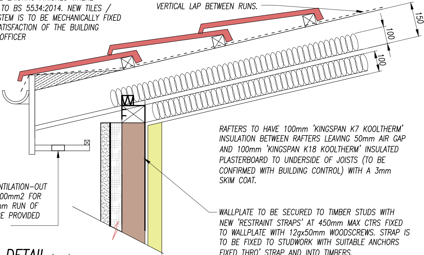
EAVES DETAIL (1:10) (NEW ROOF TO FRONT GABLED DORMER)
