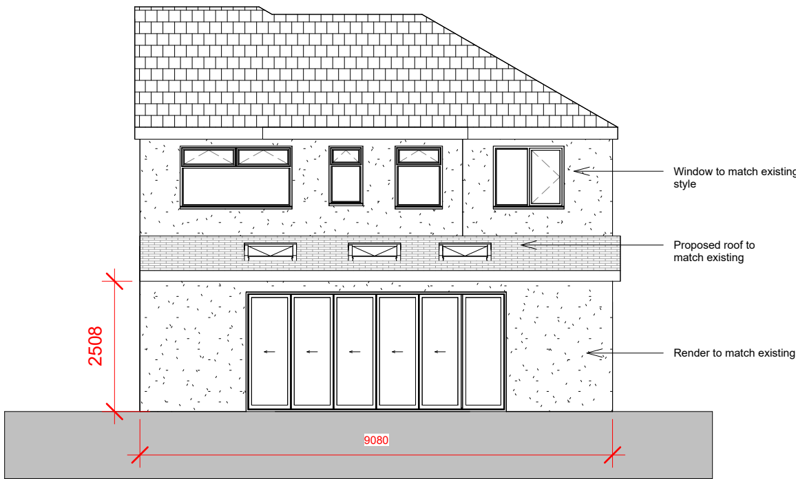
Rear Elevation 1 : 100
