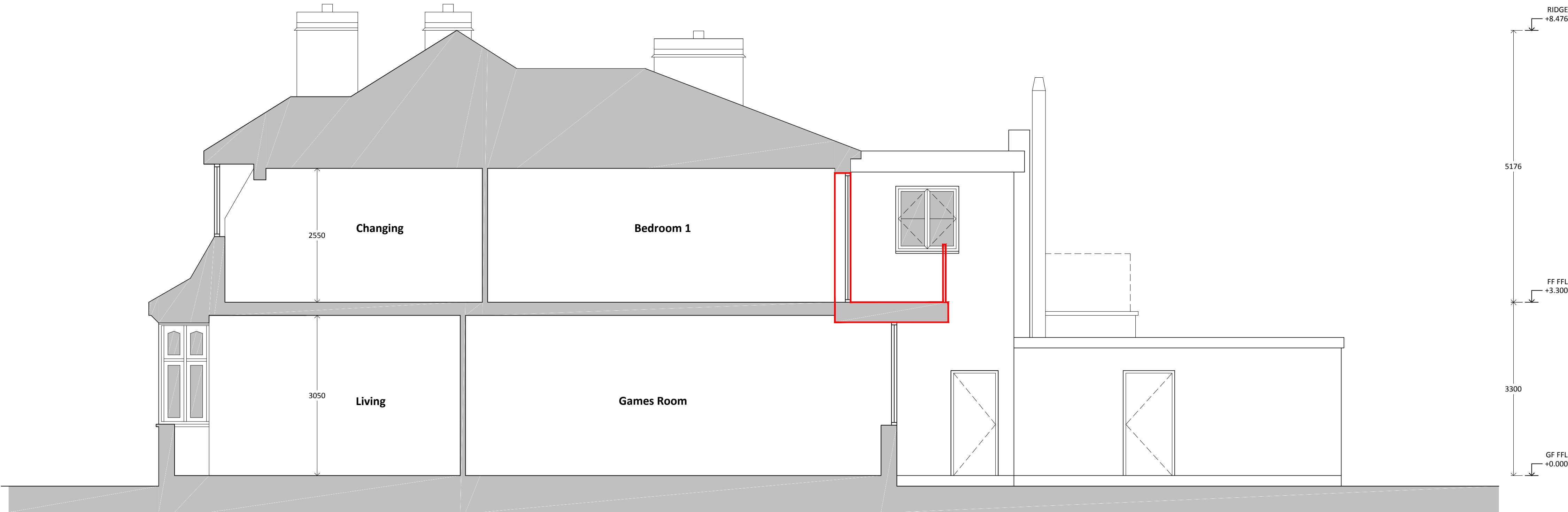
PROPOSED SECTION A-A SCALE 1:50
