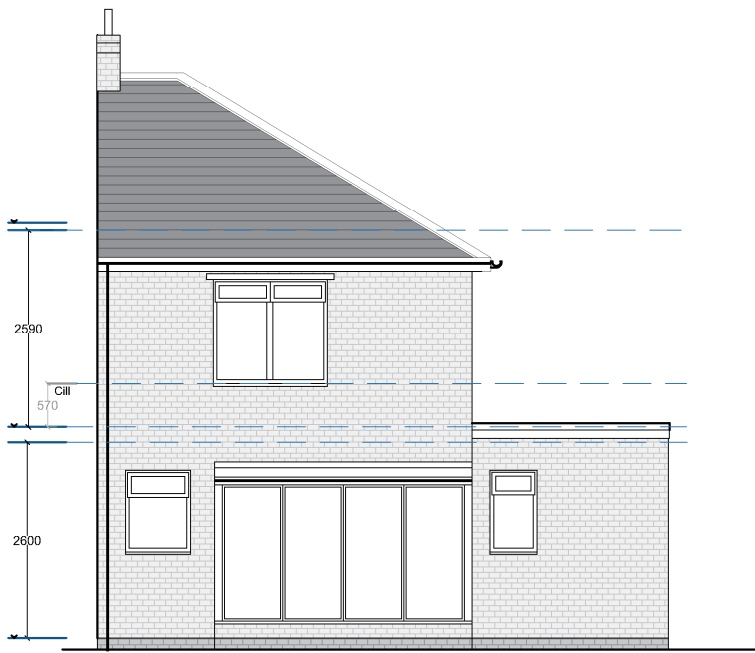
EXISTING REAR ELEVATION (Scale 1:100) SCALE BAR - (mm) 500 1000 2000
