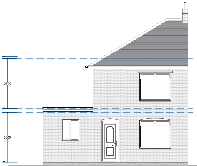
EXISTING FRONT ELEVATION (Scale 1:100) SCALE BAR - (mm) 500 1000 2000
