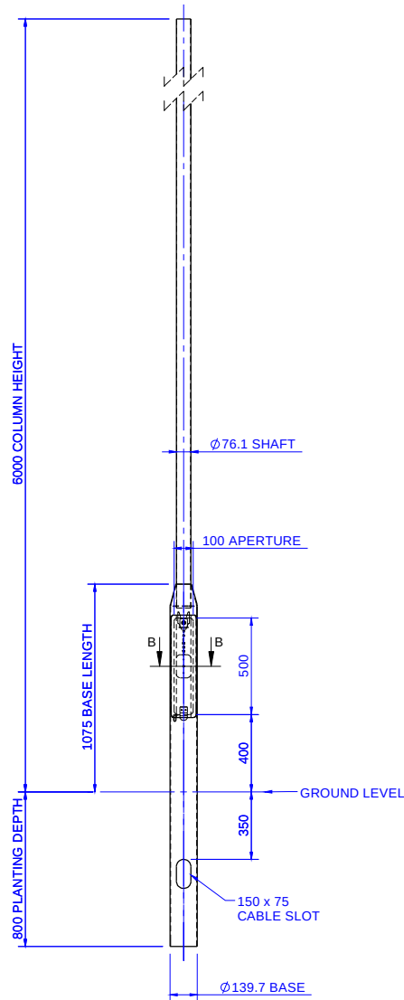
ELEVATION ON COLUMN SCALE 1:25
