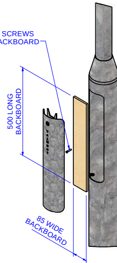
EXPLODED VIEW ON DOOR EQUIPMENT
