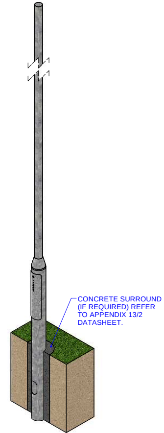
ISOMETRIC
