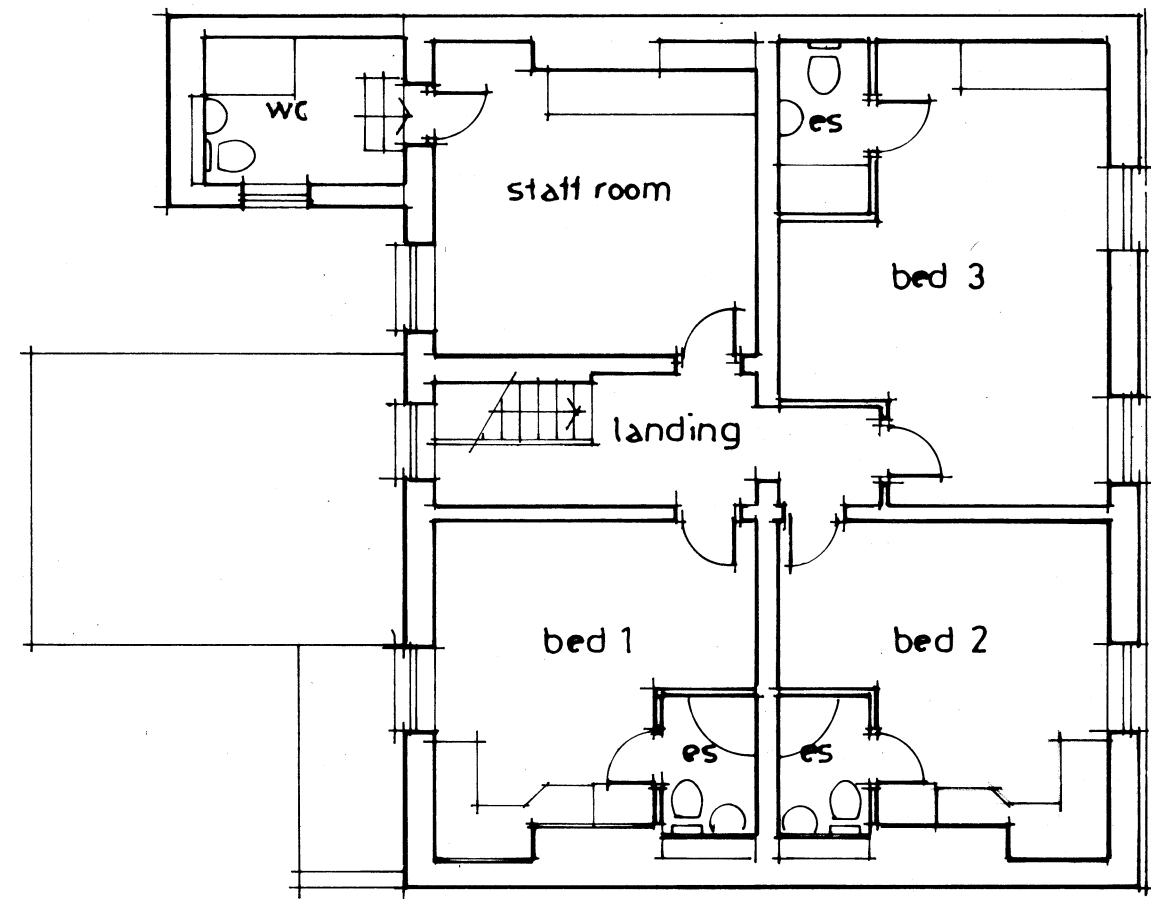
FIRST FLOOR PLAN (EXISTING) 1:100 surveyed Feb 2024
