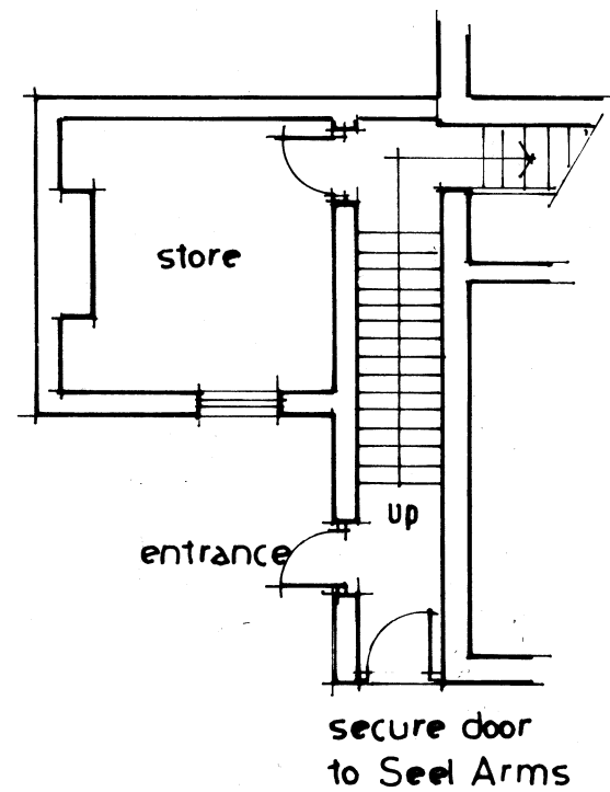
MEZZANINE & PART GROUND FLOOR PLAN (EXISTING) 1:100 surveyed Feb 2024
