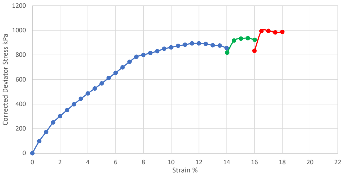
CORRECTED DEVIATOR STRESS vs AXIAL STRAIN
