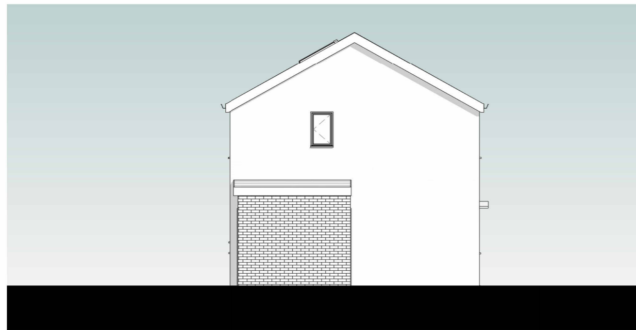
3 Existing Side Elevation 1 : 100
