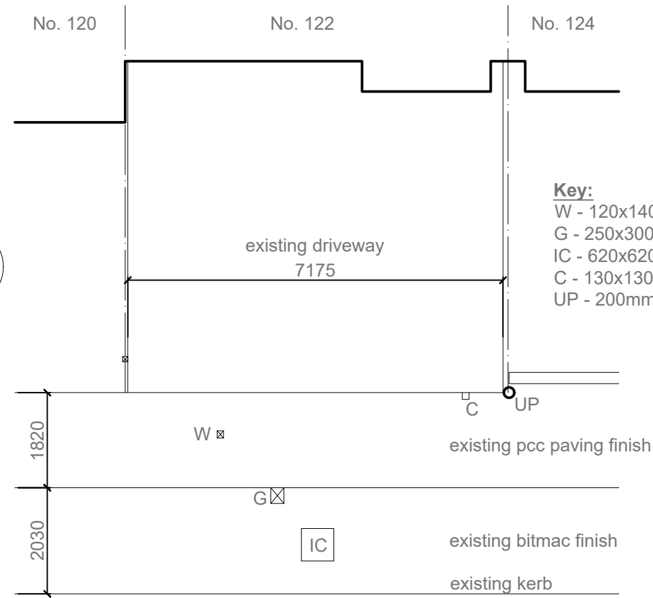
Existing layout @ 1:100 scale
