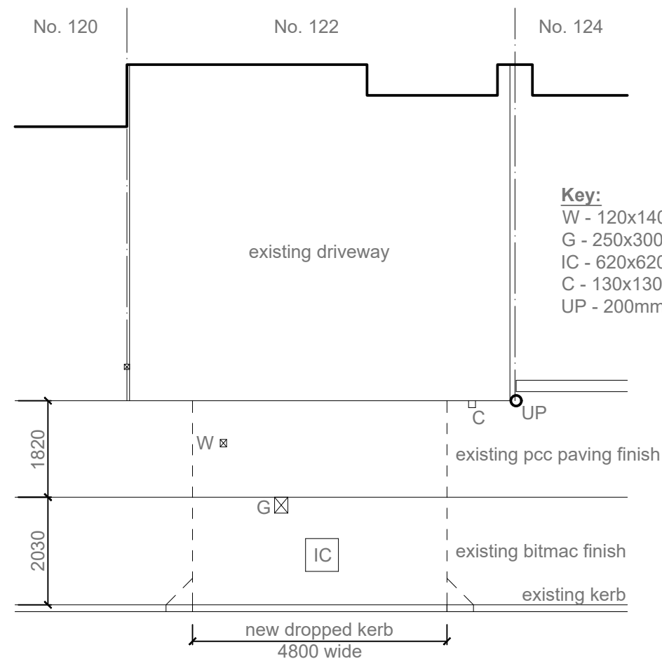
Proposed layout @ 1:100 scale
