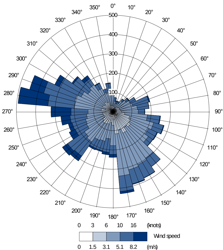
Figure 4-2. Liverpool 2019 Wind Rose
