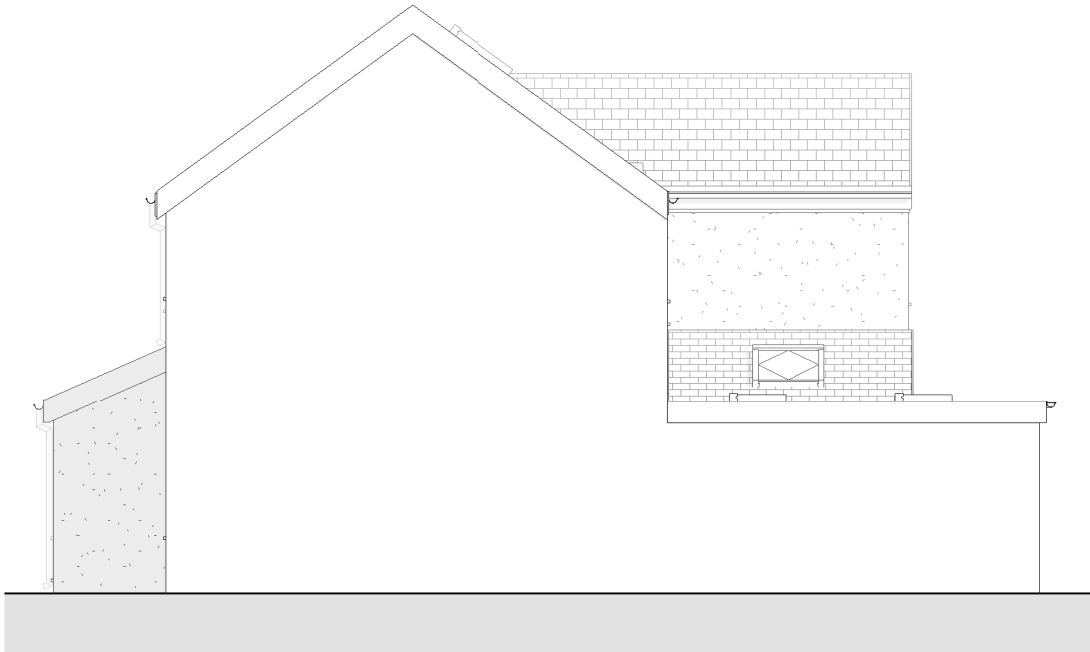
Proposed Side Elevation (No. 19)
