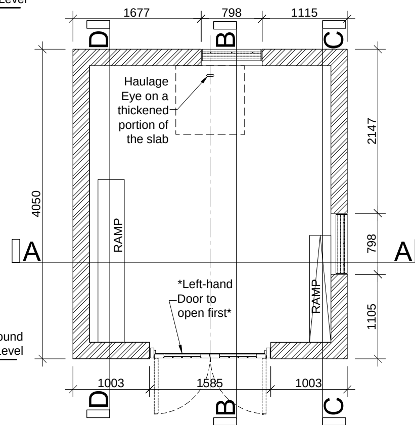
Section Key Plan
