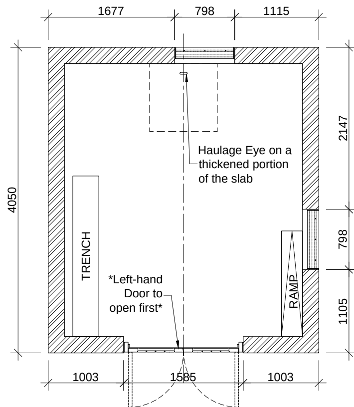
Wall Plan
