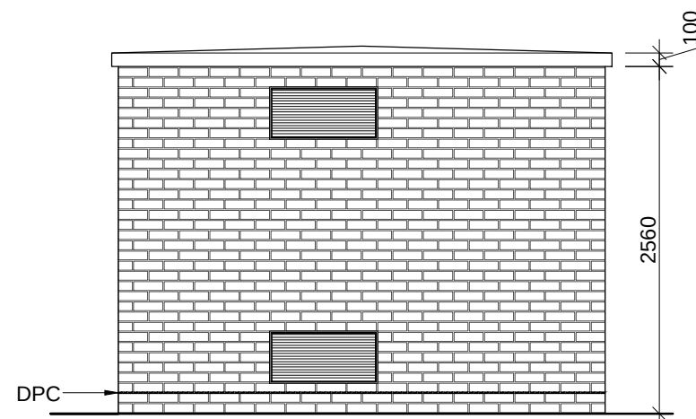
Rear (North) Elevation
