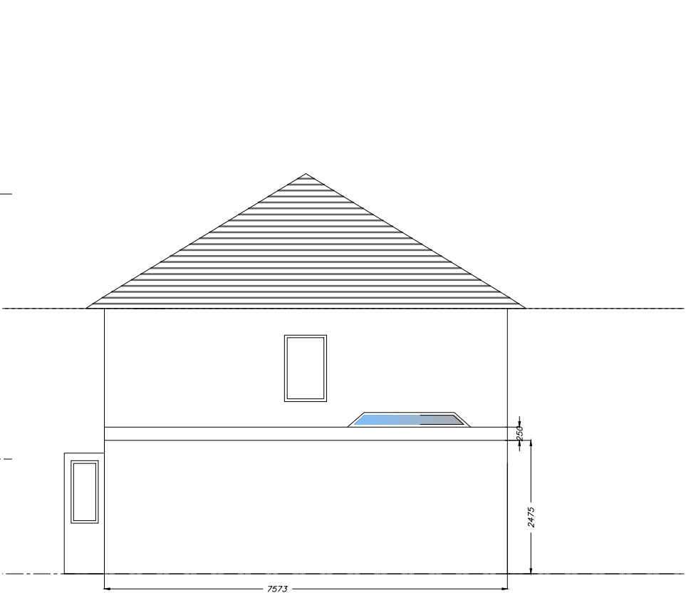
Proposed RH/Side Elevation
