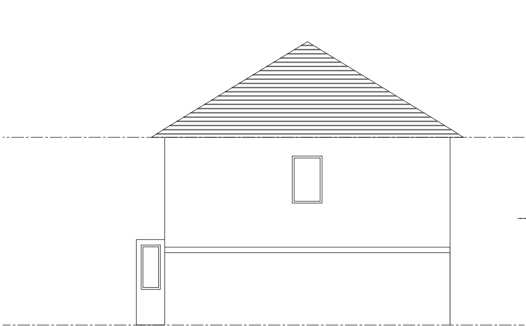
Existing RH/Side Elevation
