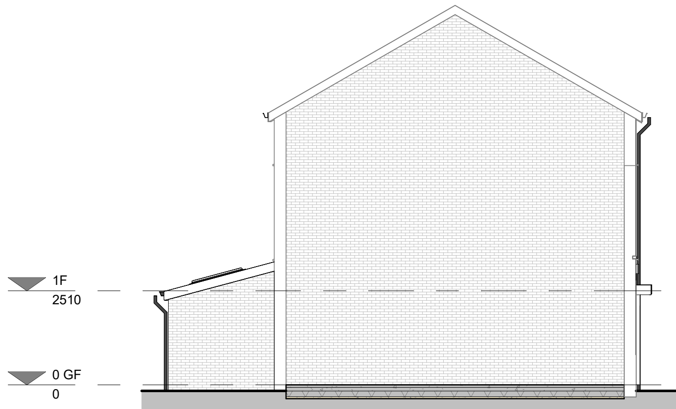
SIDE ELEVATION II (West Facing)
