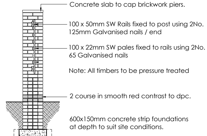
Boundary Wall Section
