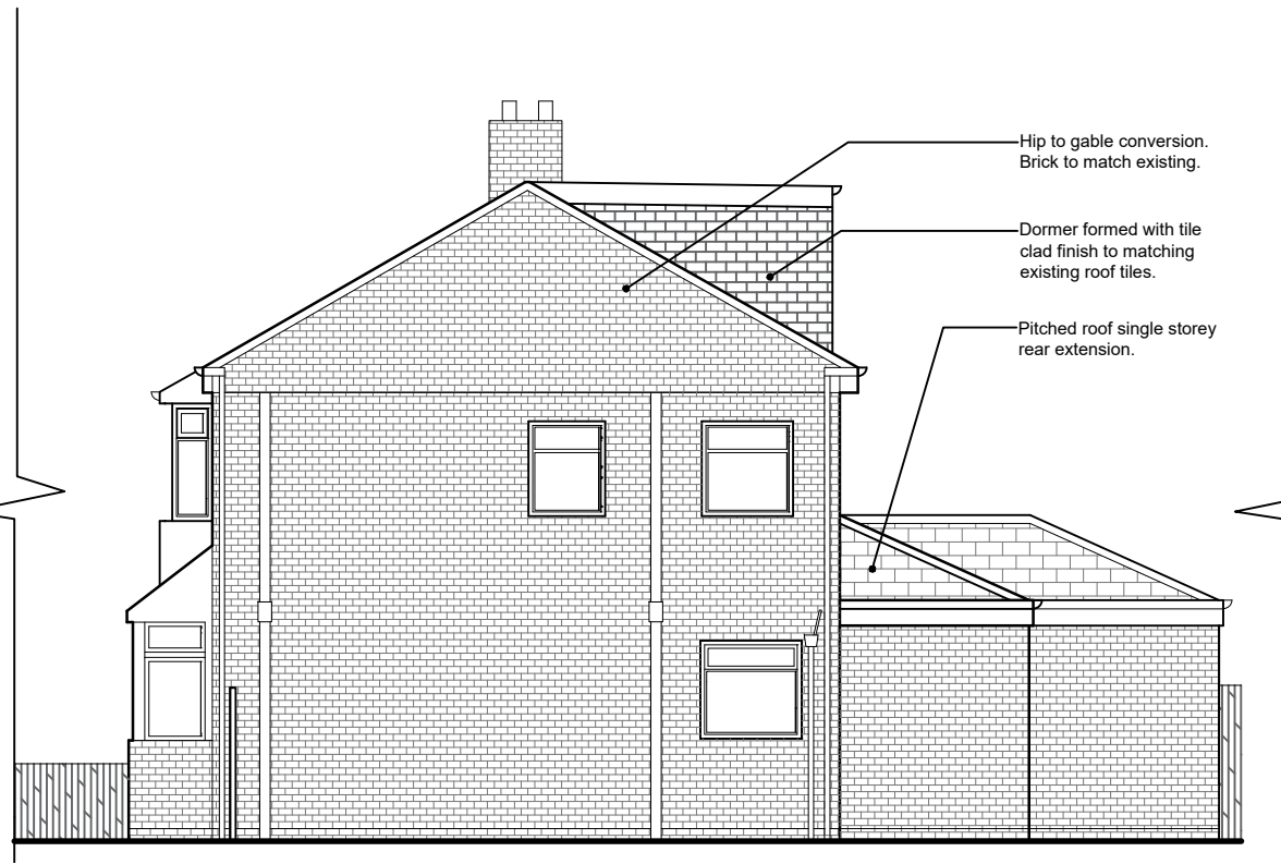
PROPOSED ELEVATION B-B SCALE 1:100
