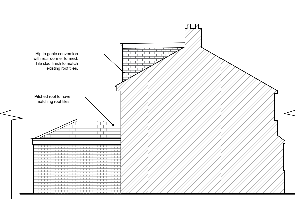
PROPOSED ELEVATION D-D SCALE 1:100
