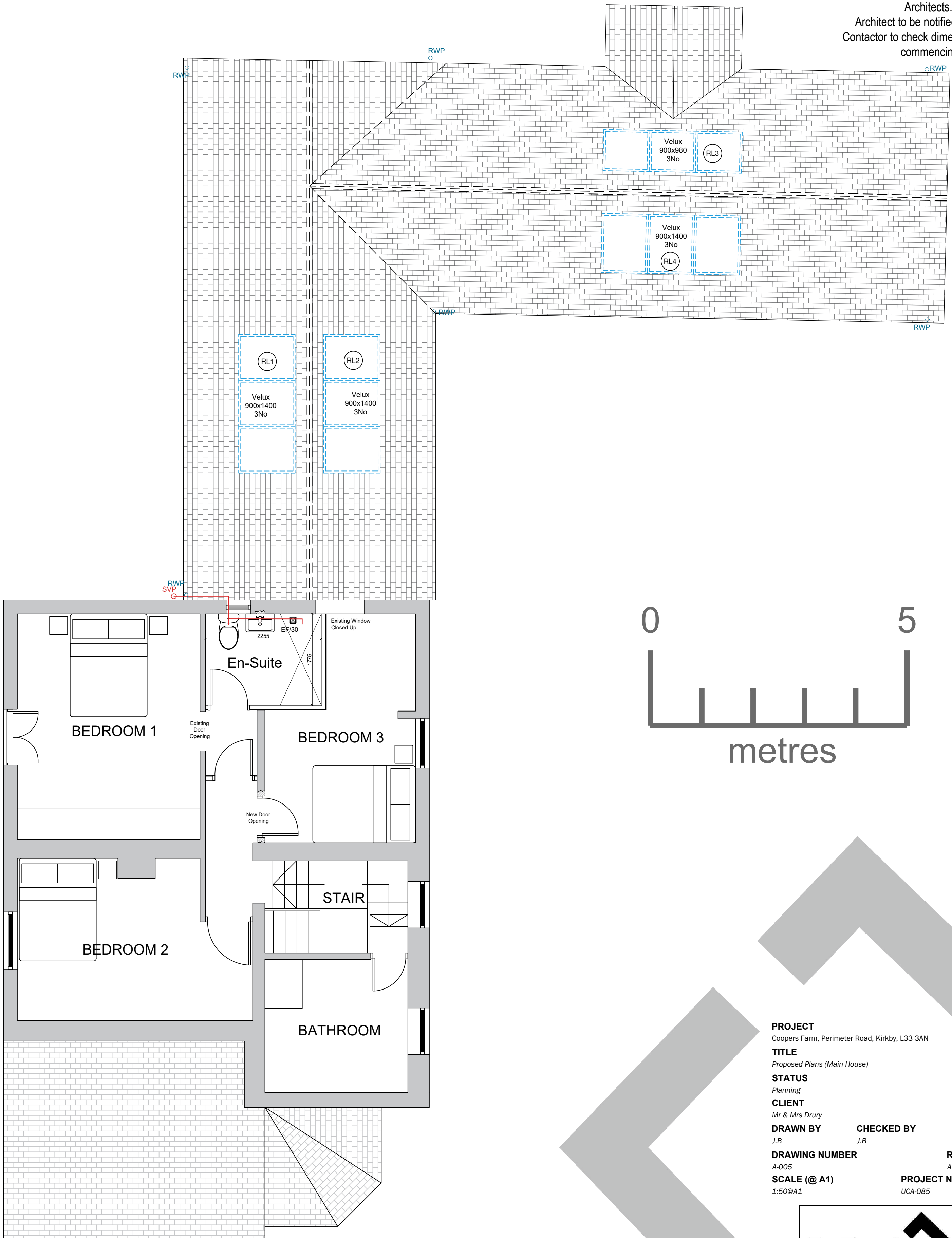
PROPOSED FIRST FLOOR 1:50
