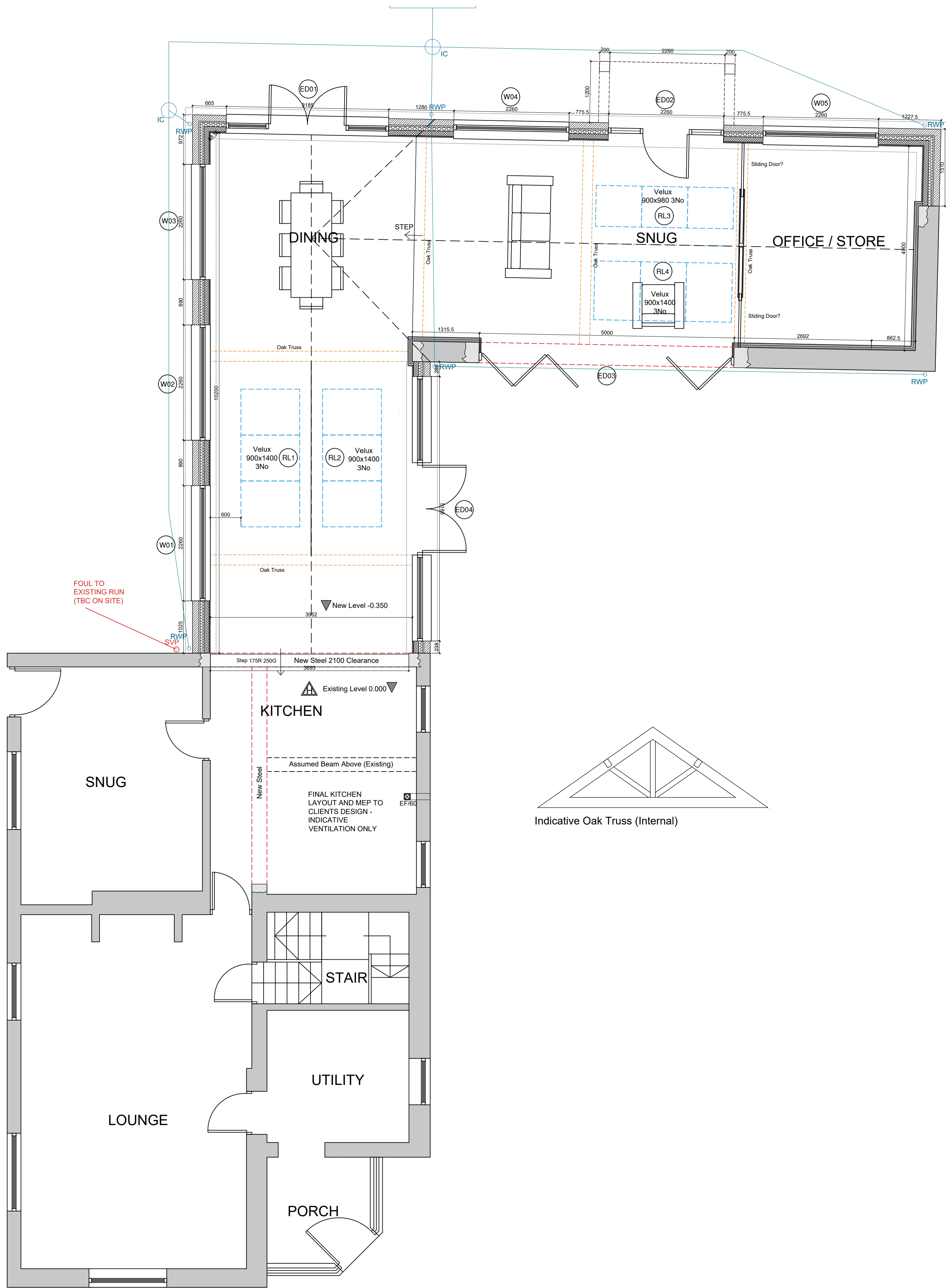
PROPOSED GROUND FLOOR 1:50
