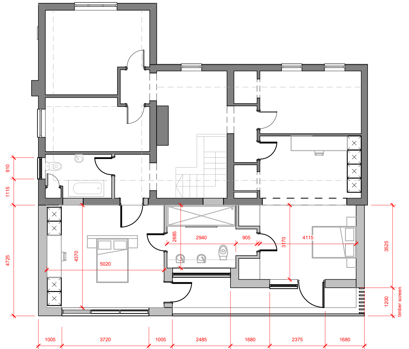
Proposed - 1F 1 : 100
