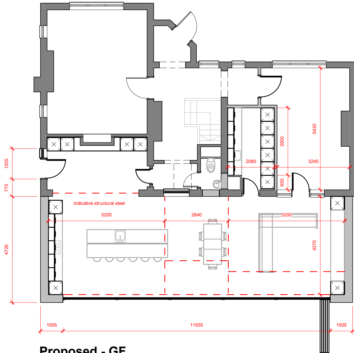
Proposed - GF 1 : 100
