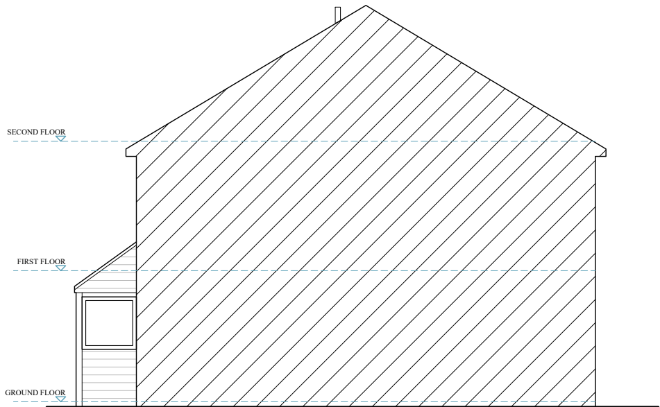
PROPOSED NORTH SIDE ELEVATION
