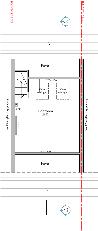
EXISTING SECOND FLOOR PLAN
